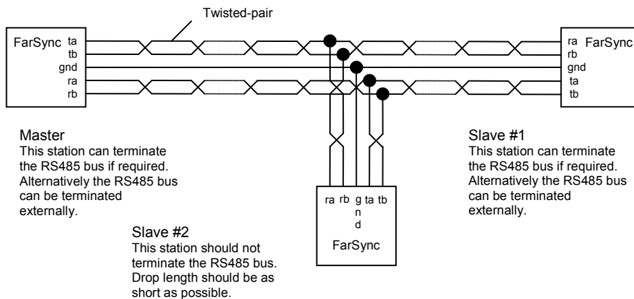
Simple 4-wire multidrop RS485 network with signal ground
